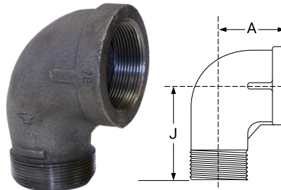
Fig. 1103, 1103R 90° Straight Street Elbow (Class 150 Standard) 90° Reducing Street Elbow (Class 150 Standard)
