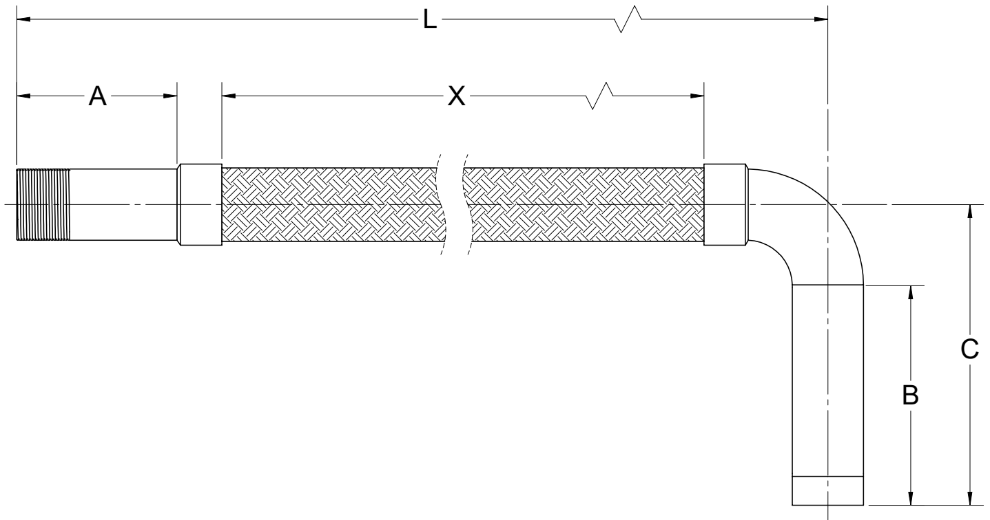
Fig. 20XXHE Dimensions & Model Number
