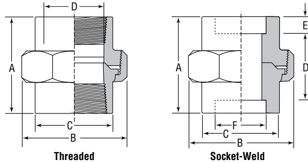
Figure 2127 Threaded Union
