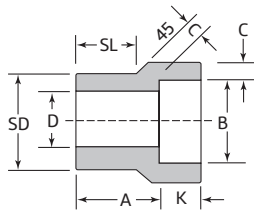
Type 1 – Reducer Insert Fig. 2159
