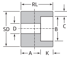
Type 2 – Reducer Insert Fig. 2179
