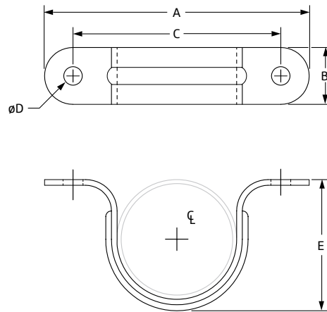
Fig. 266: Dimensions (in) • Weight (lbs)
