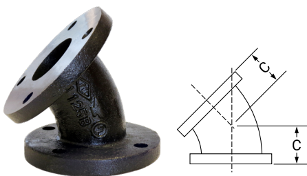
Fig. 802 45° Flanged Elbow (Class 125 Standard)
