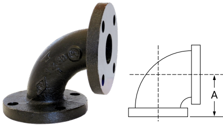
Fig. 801 90° Flanged Elbow (Class 125 Standard)
