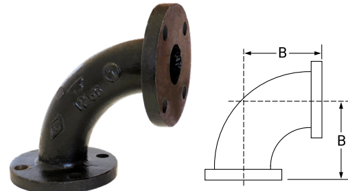
Fig. 804 90° Long Radius Flanged Elbow (Class 125 Standard)
