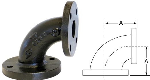
Fig. 803 90° Reducing Flanged Elbow (Class 125 Standard)
