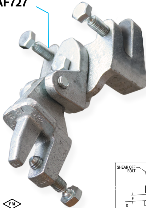
FIG. AF727: Dimensions and Weights
