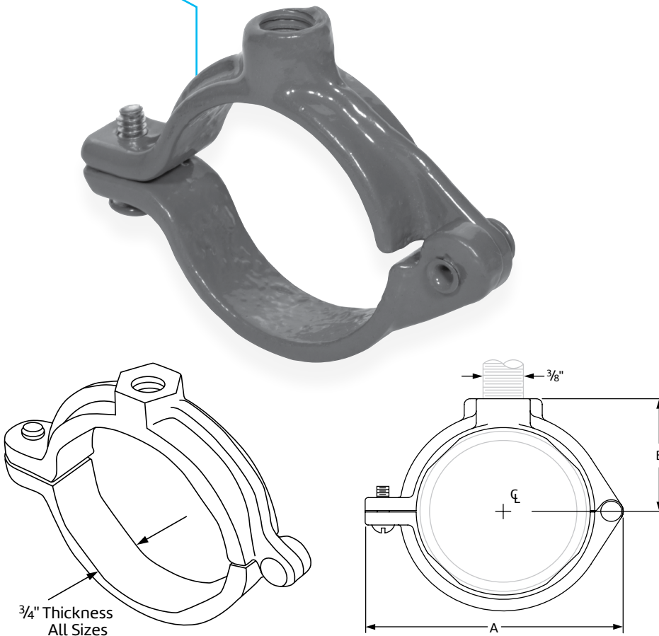
Fig. CT-138R: Dimensions (in) • Loads (lbs) • Weight (lbs)
