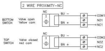
Old Style Board Wiring
