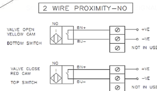
New Style Board Wiring
