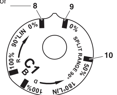
Cam Marking.eps
