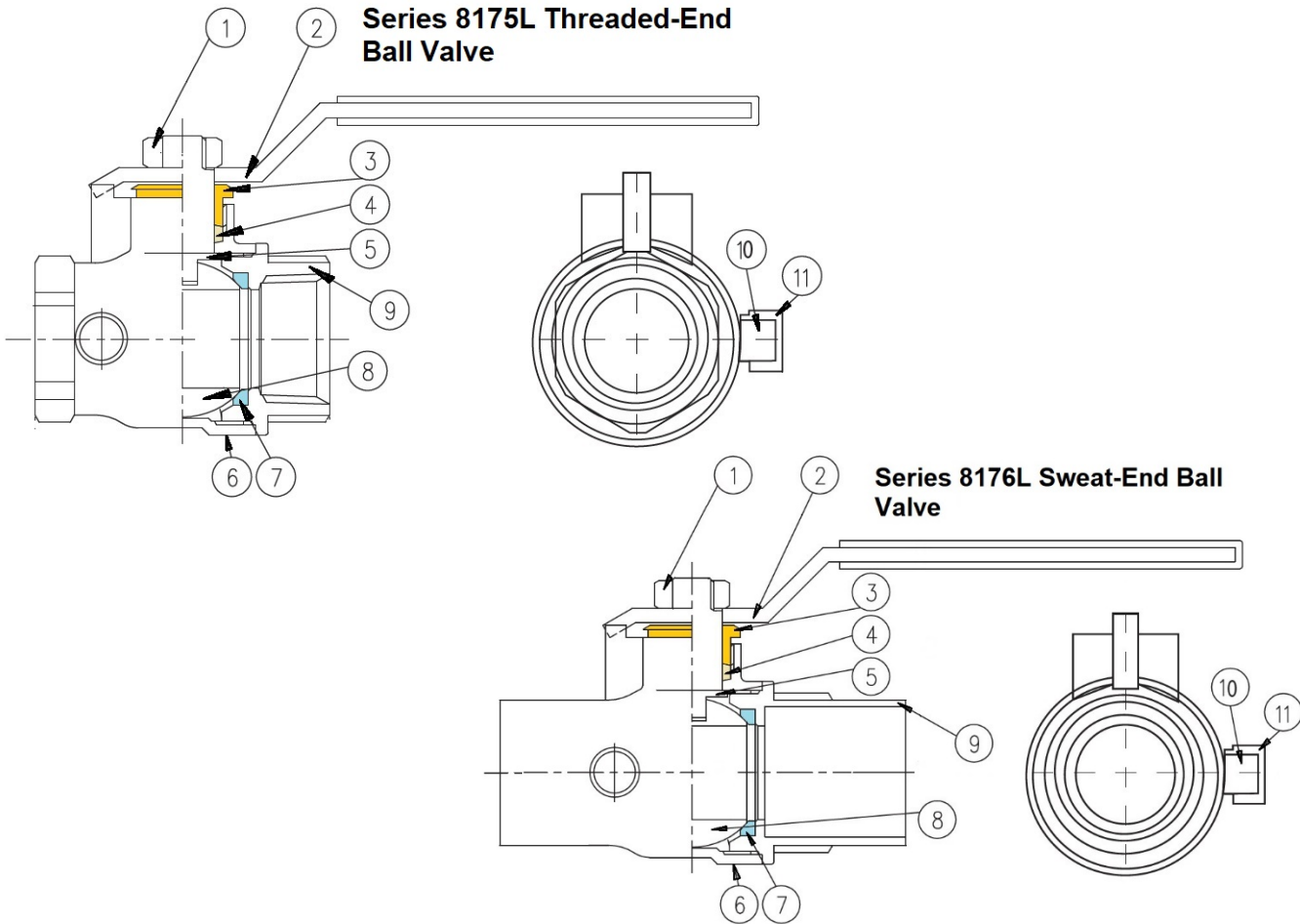
Figure 1 – SCI Series 8175L & 8176L 2-Piece Brass Ball Valves with Drain
