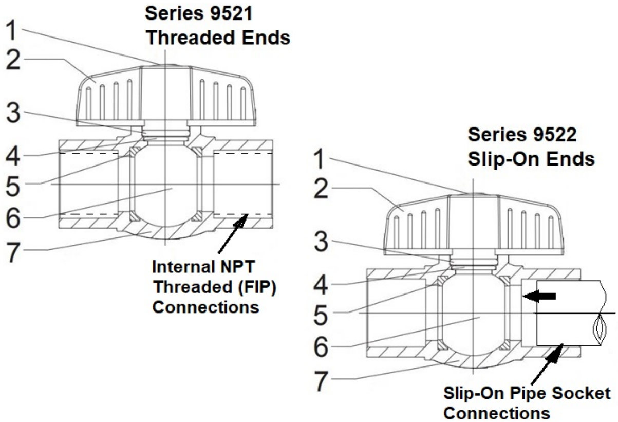
Figure 1 – SCI Series 9521 & 9522 PVC Ball Valve
