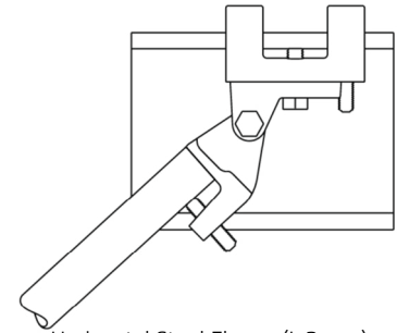
Horizontal Steel Flange (I-Beam) Seismic Load Parallel to the Flange
